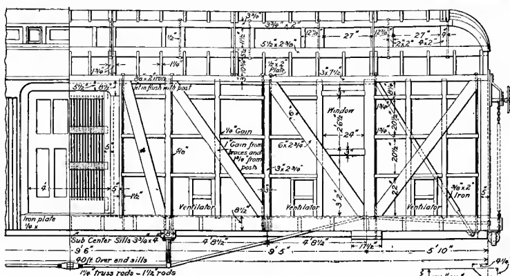
Fig. 584. Half Side Elevation of Framing.
